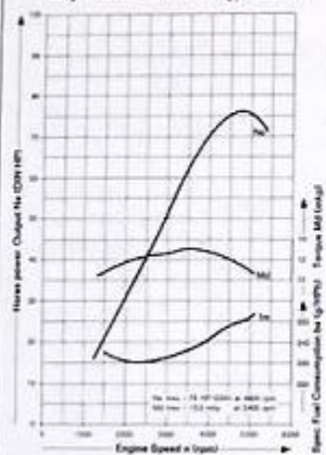
Full-power Performance Type 914 - 1.8
