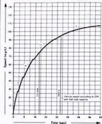
Acceleration Curve Type 914 - 1.8
